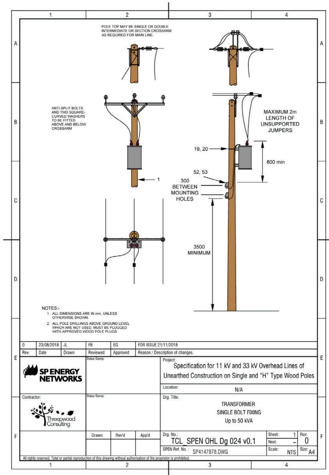
22.24 Figure 24 General Arrangement Transformer Single Bolt Fixing up to 50kVA (Drawing No. SP4147878)
